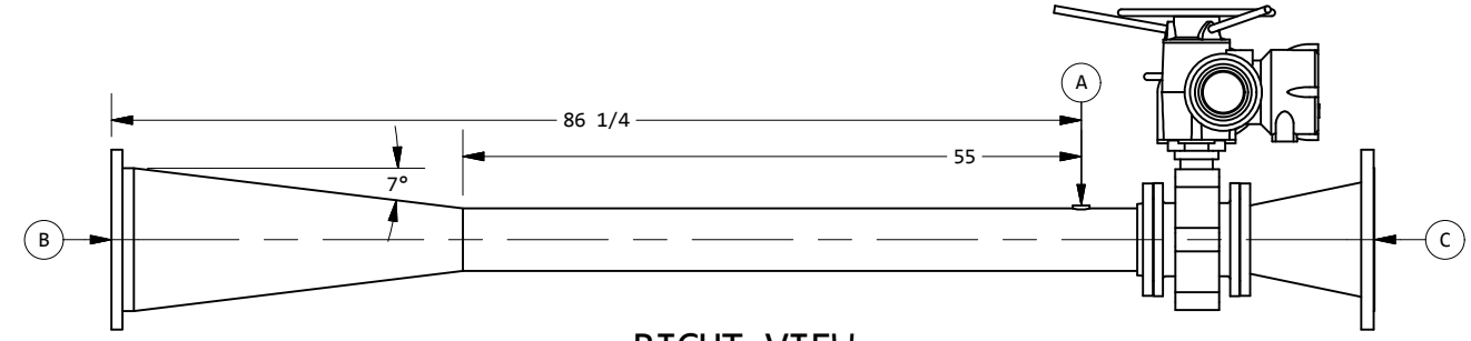
RIGHT VIEW
